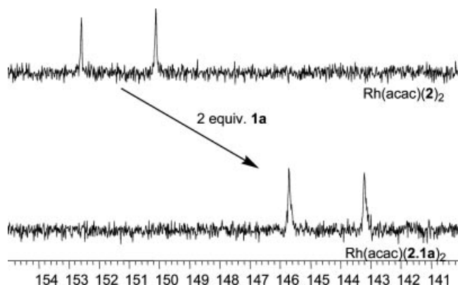
Figure 3. ^{31}\text{P} NMR spectra before (above) and after (below) addition of two equivalents of zinc(II) meso,meso,meso,meso -tetraphenylporphyrin ( 1a ) to the complex [\text{Rh}(\text{acac})(\mathbf{2})_2] .
