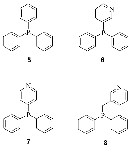
Figure 4. Various ligand building blocks used to construct supra-molecular ligands.
