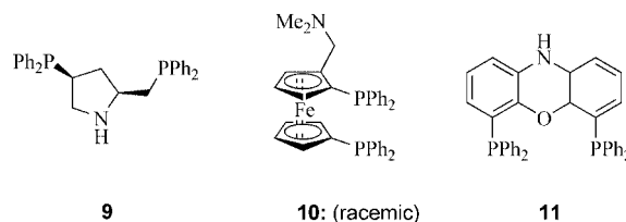
Figure 6. Various diphosphane ligand building blocks that were used to construct supramolecular ligands via nitrogen coordination to zinc(II) porphyrins.
