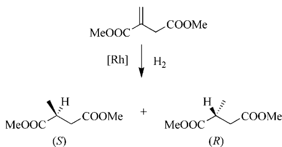
Scheme 3. The rhodium-catalyzed hydrogenation of dimethyl itaconate.
