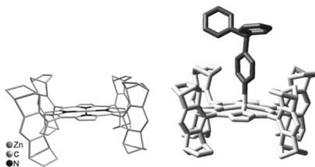
Figure 9. Crystal structure of the zinc(II) complex of meso,meso-meso-tetrakis(octahydro-1,4:5,8-dimethanoanthryl)porphyrin ( 12a ) (left) and modeled structure of the assembly of 12a (white) and diphenyl(4-pyridyl)phosphane ( 7 ) (dark gray, right).
