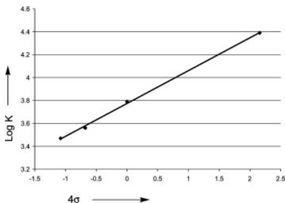
Figure 5. Plot log K vs. 4\sigma (sigma para ) for the assembly of zinc(II) porphyrin complexes 1a–d and diphenyl(4-pyridyl)phosphane (7).
