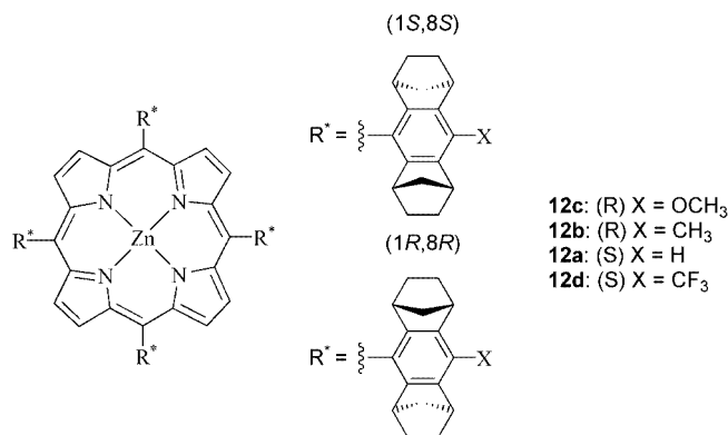
Figure 8. Various chiral porphyrin building blocks used to construct supramolecular ligands.
