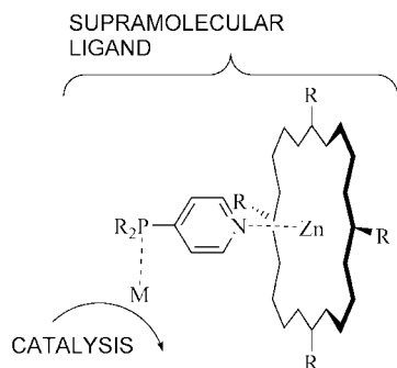
Figure 1. Schematic representation of the assembly of a phosphorus ligand on a zinc(II) porphyrin template molecule.
