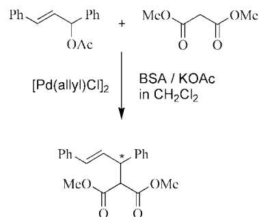
Scheme 4. Palladium-catalyzed allylic alkylation.
