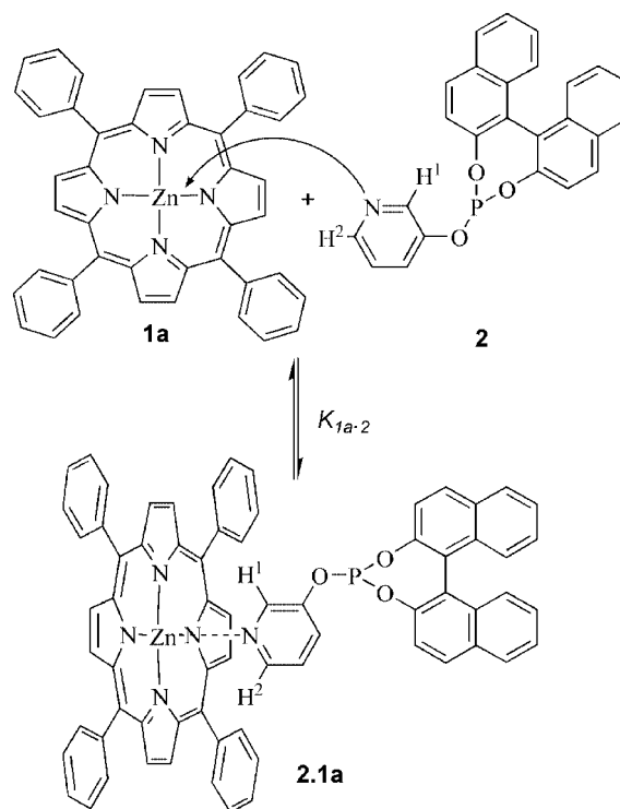
Scheme 1. Assembly of (S)-(1,1'-binaphthyl-2,2'-diyl) (3-pyridyl) phosphite ( 2 ) on zinc(II) meso,meso,meso,meso -tetraphenylporphyrin ( 1a ).
