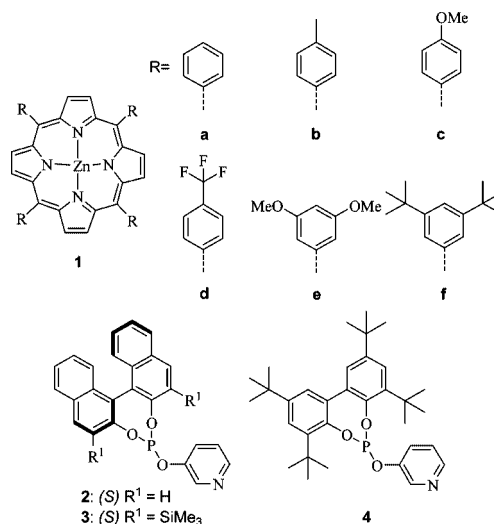
Figure 2. Various building blocks used to construct supramolecular ligands.
