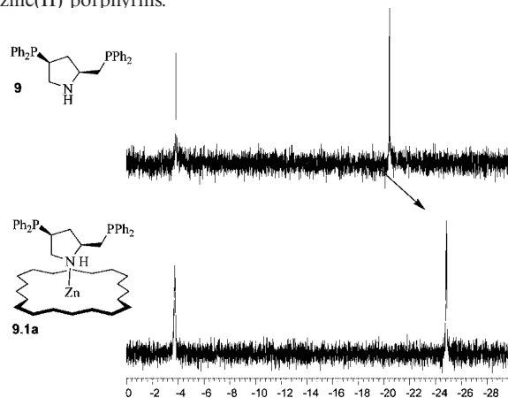
Figure 7. 31 P NMR spectra of (2 S ,4 S )-(–)-4-(diphenylphosphanyl)-2-(diphenylphosphanylmethyl)pyrrolidine ( 9 ) in absence (above) and presence (below) of zinc(II) porphyrin 1a .
