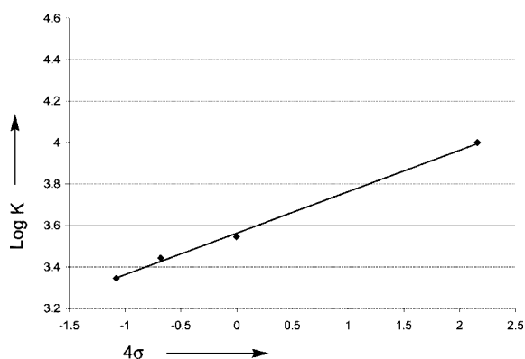
Figure 10. Plot \log K vs. 4\sigma for the reaction of zinc(II) porphyrins 12a–d and diphenyl(4-pyridyl)phosphane ( 7 ).
